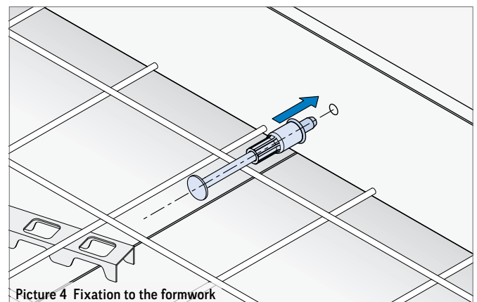
Picture 4 Fixation to the formwork
